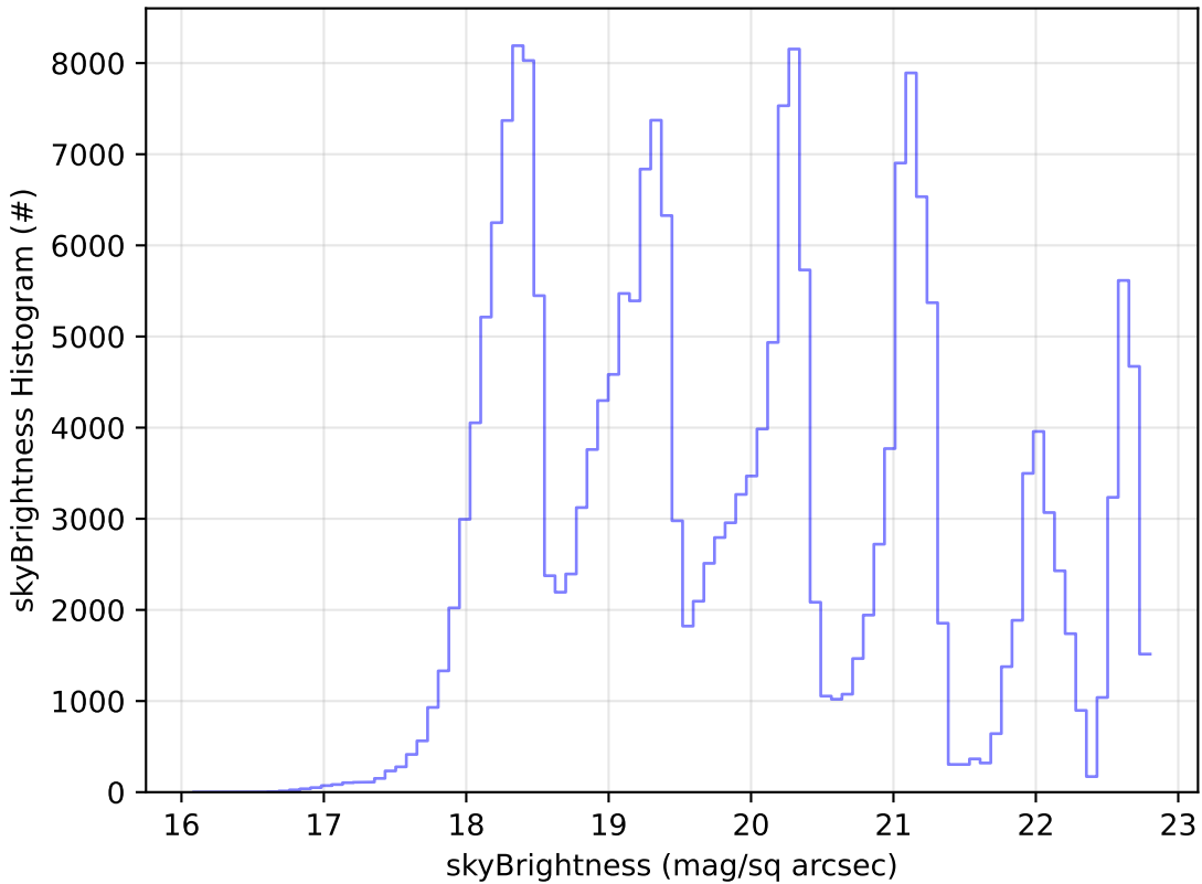
too_elab_r128_d3_gz_v3.4_10yrs Yr 1 all bands: skyBrightness Histogram
