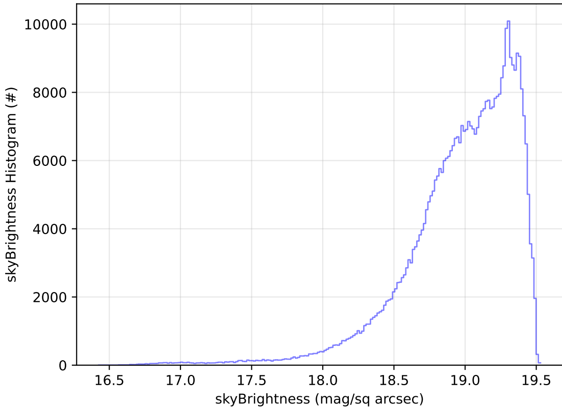
too_elab_r128_d3_gz_v3.4_10yrs WFD z band: skyBrightness Histogram
