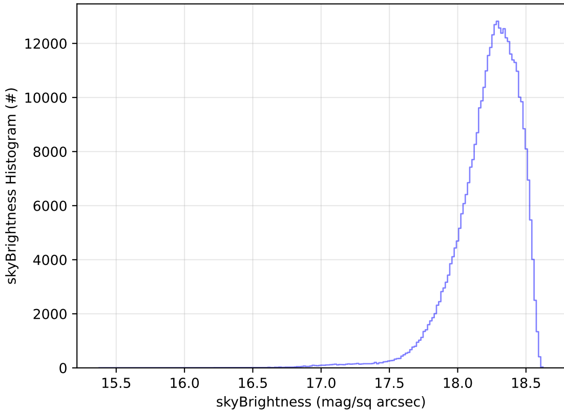
too_elab_r128_d3_gz_v3.4_10yrs WFD y band: skyBrightness Histogram
