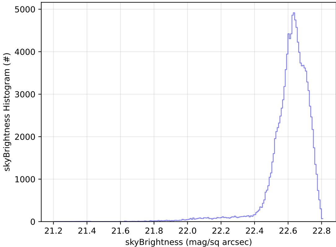
too_elab_r128_d3_gz_v3.4_10yrs WFD u band: skyBrightness Histogram
