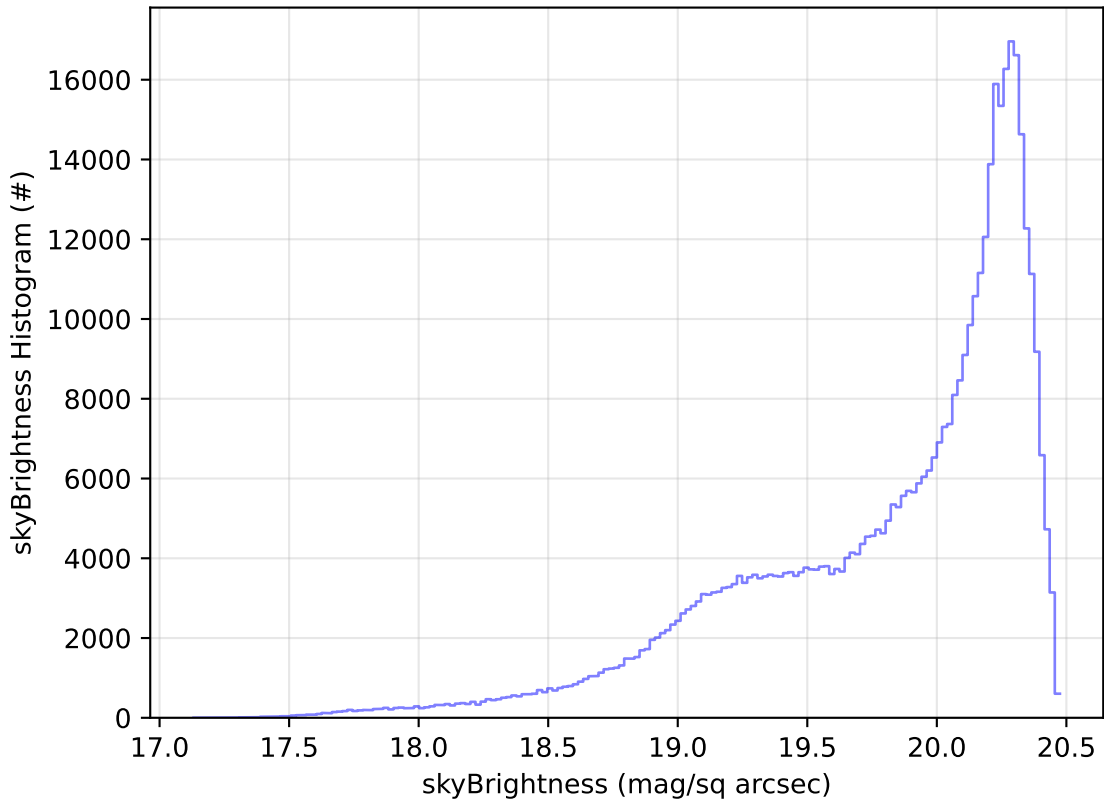
too_elab_r128_d3_gz_v3.4_10yrs WFD i band: skyBrightness Histogram
