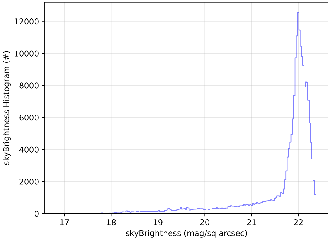
too_elab_r128_d3_gz_v3.4_10yrs WFD g band: skyBrightness Histogram
