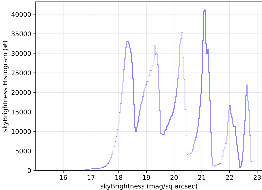
too_elab_r128_d3_gz_v3.4_10yrs WFD all bands: skyBrightness Histogram
