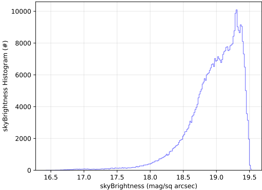
too_elab_r128_d3_gz_v3.4_10yrs All sky z band: skyBrightness Histogram
