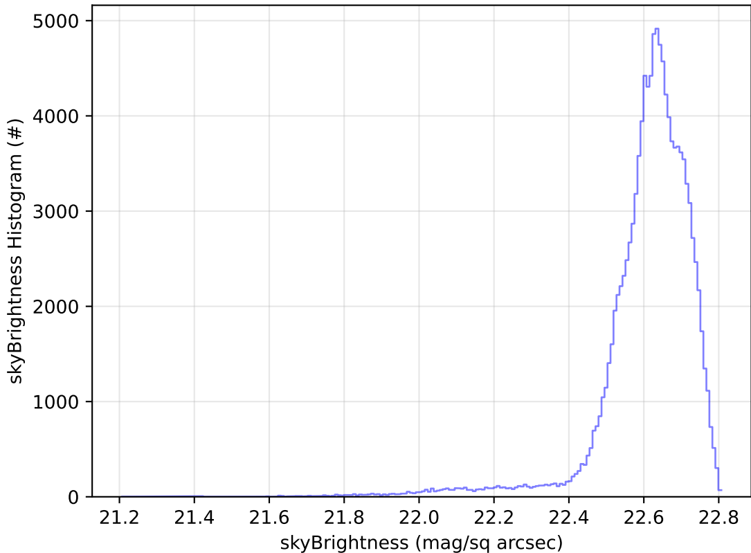
too_elab_r128_d3_gz_v3.4_10yrs All sky u band: skyBrightness Histogram
