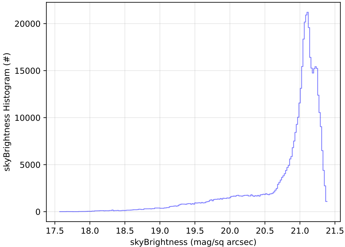
too_elab_r128_d3_gz_v3.4_10yrs All sky r band: skyBrightness Histogram
