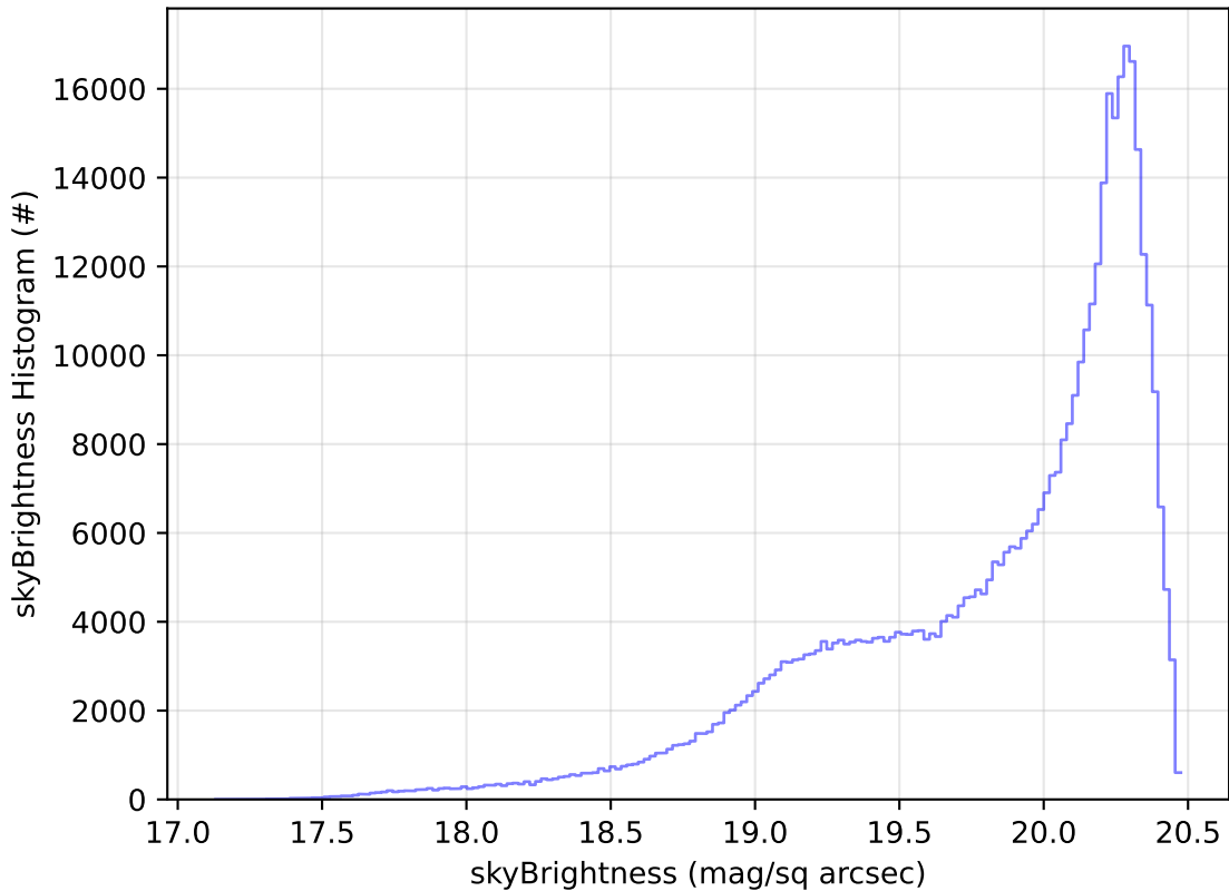
too_elab_r128_d3_gz_v3.4_10yrs All sky i band: skyBrightness Histogram
