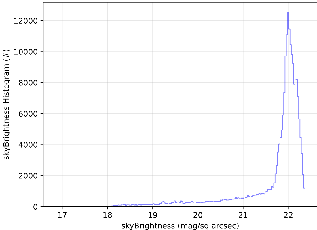
too_elab_r128_d3_gz_v3.4_10yrs All sky g band: skyBrightness Histogram
