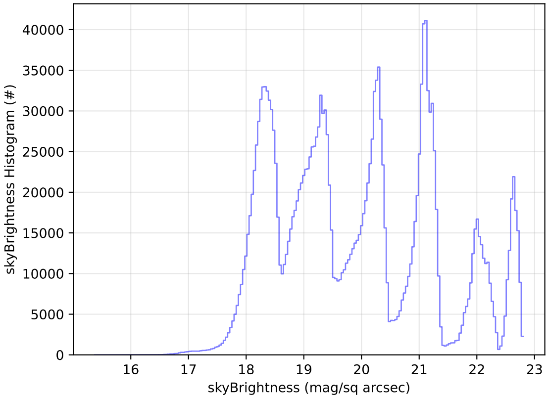
too_elab_r128_d3_gz_v3.4_10yrs All sky all bands: skyBrightness Histogram
