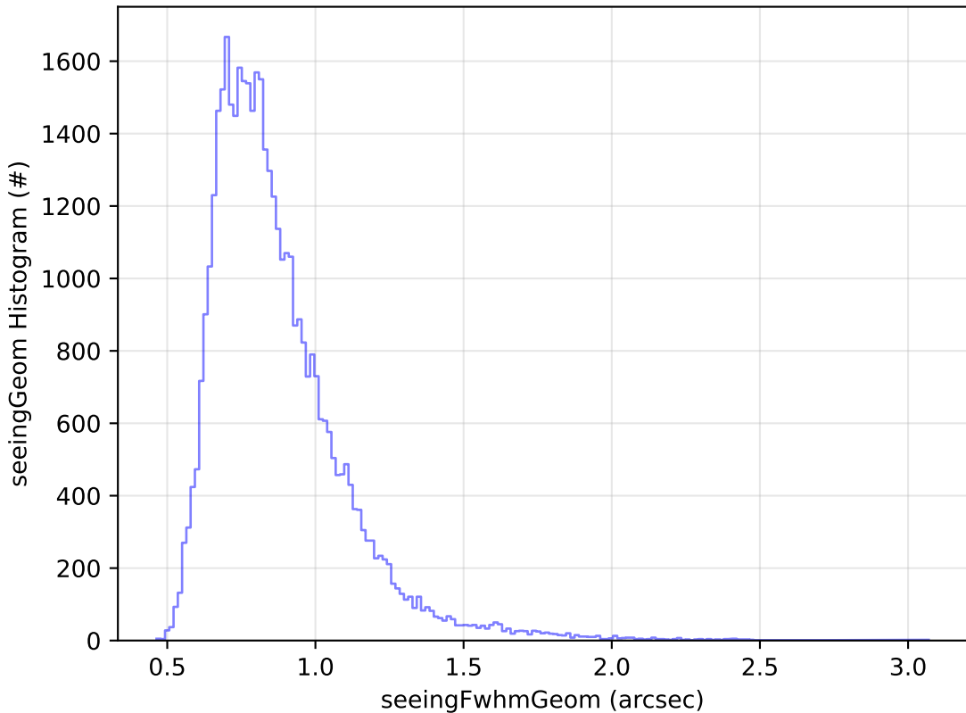
too_elab_r128_d3_gz_v3.4_10yrs Yr 1 z band: seeingGeom Histogram
