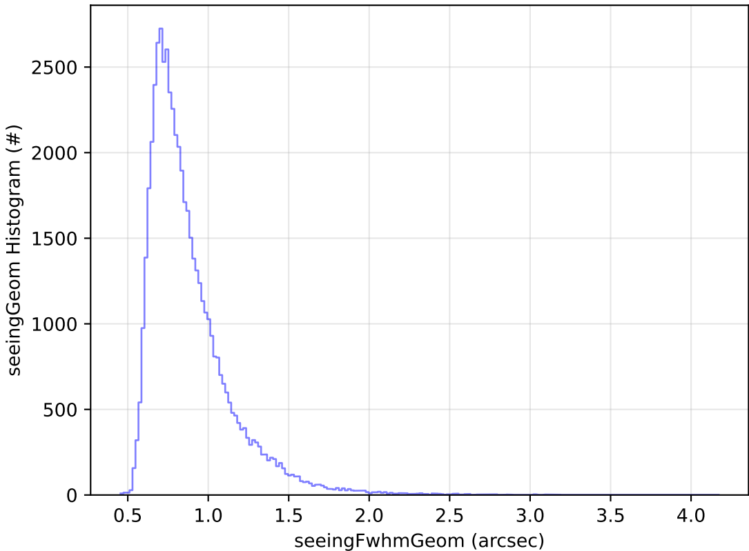
too_elab_r128_d3_gz_v3.4_10yrs Yr 1 i band: seeingGeom Histogram
