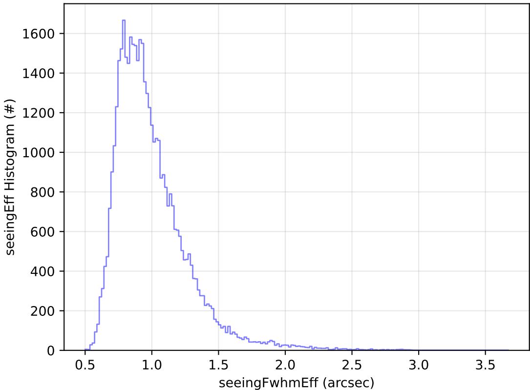
too_elab_r128_d3_gz_v3.4_10yrs Yr 1 z band: seeingEff Histogram
