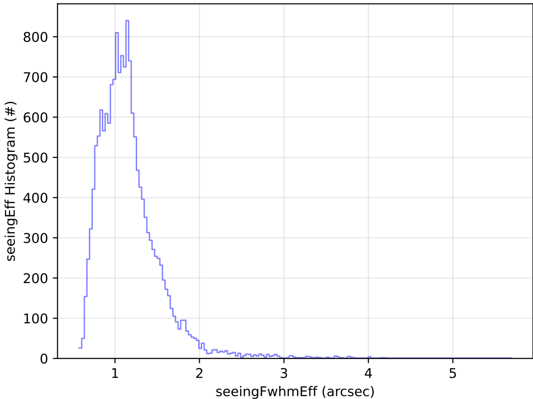
too_elab_r128_d3_gz_v3.4_10yrs Yr 1 u band: seeingEff Histogram
