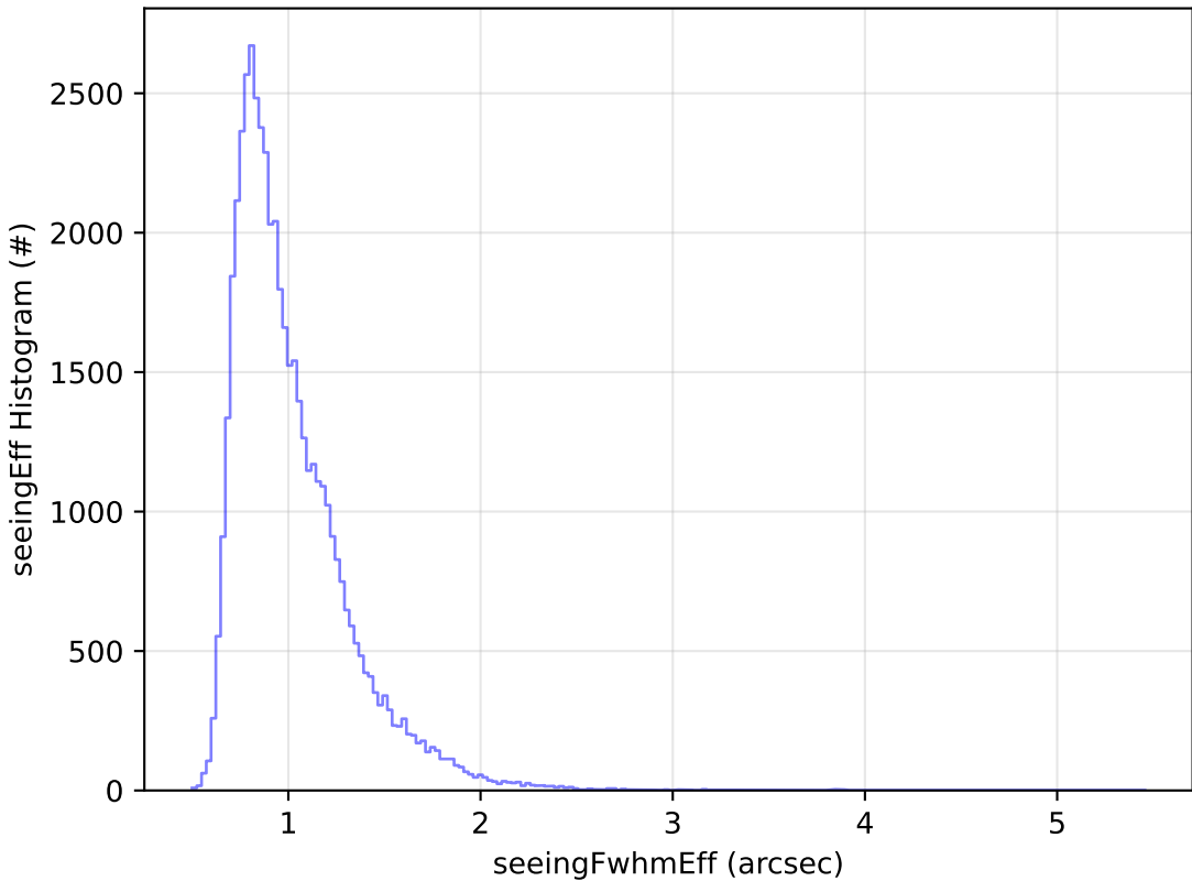
too_elab_r128_d3_gz_v3.4_10yrs Yr 1 r band: seeingEff Histogram
