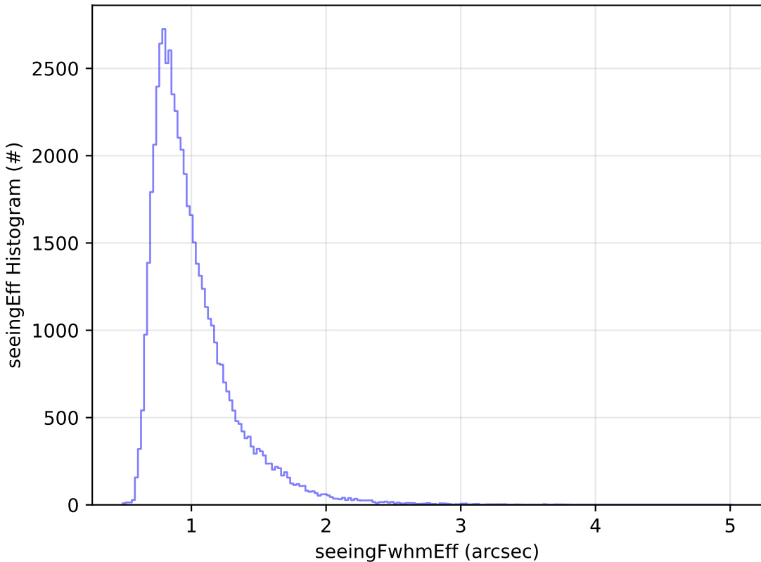
too_elab_r128_d3_gz_v3.4_10yrs Yr 1 i band: seeingEff Histogram
