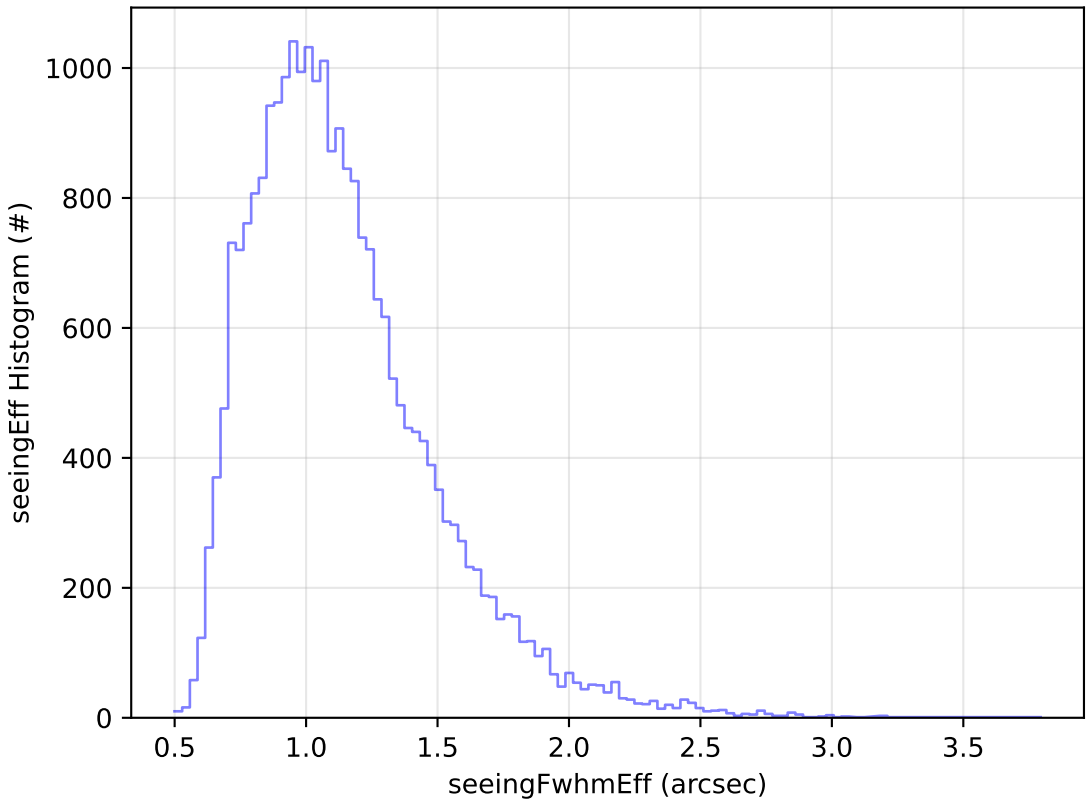
too_elab_r128_d3_gz_v3.4_10yrs Yr 1 g band: seeingEff Histogram
