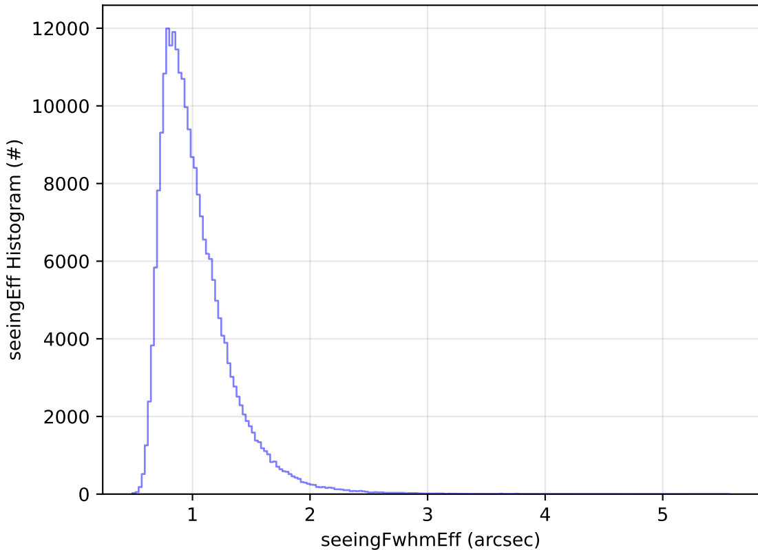
too_elab_r128_d3_gz_v3.4_10yrs Yr 1 all bands: seeingEff Histogram
