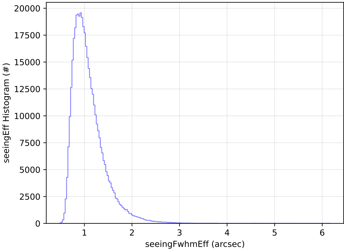
too_elab_r128_d3_gz_v3.4_10yrs WFD z band: seeingEff Histogram
