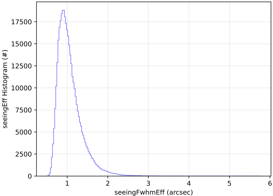
too_elab_r128_d3_gz_v3.4_10yrs WFD y band: seeingEff Histogram
