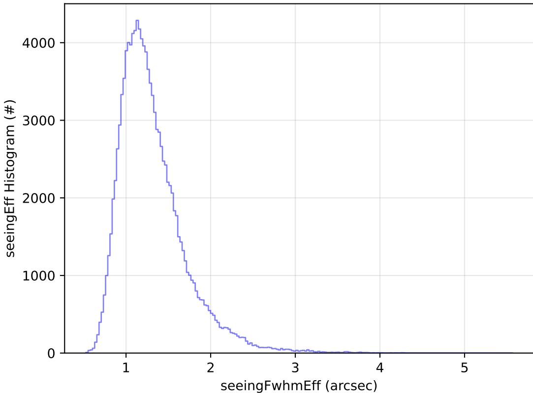
too_elab_r128_d3_gz_v3.4_10yrs WFD u band: seeingEff Histogram
