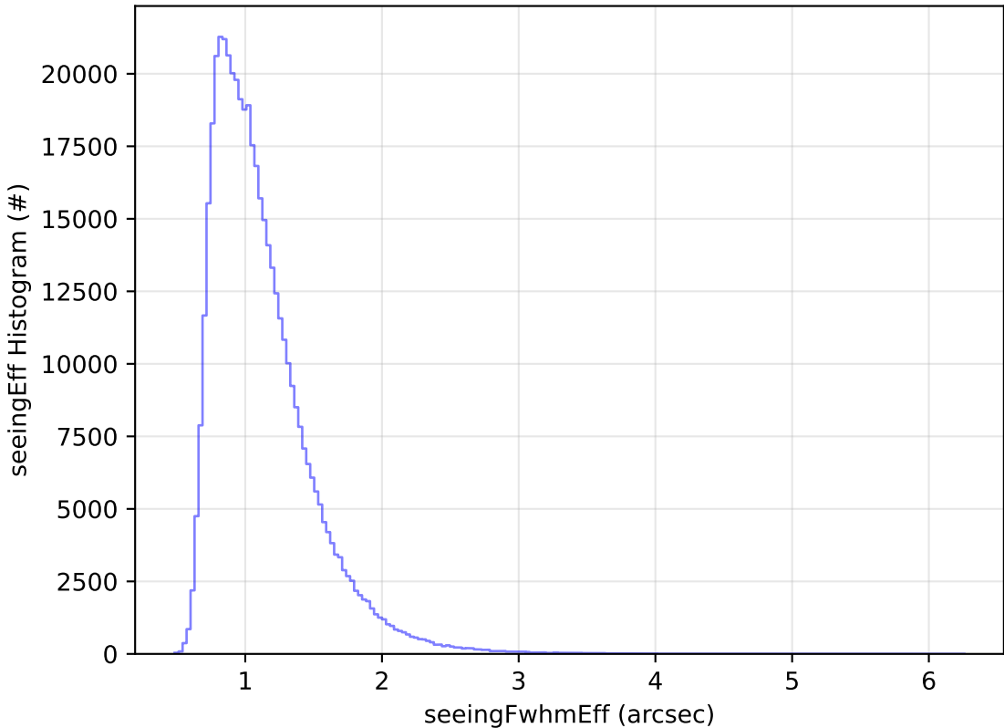
too_elab_r128_d3_gz_v3.4_10yrs WFD r band: seeingEff Histogram
