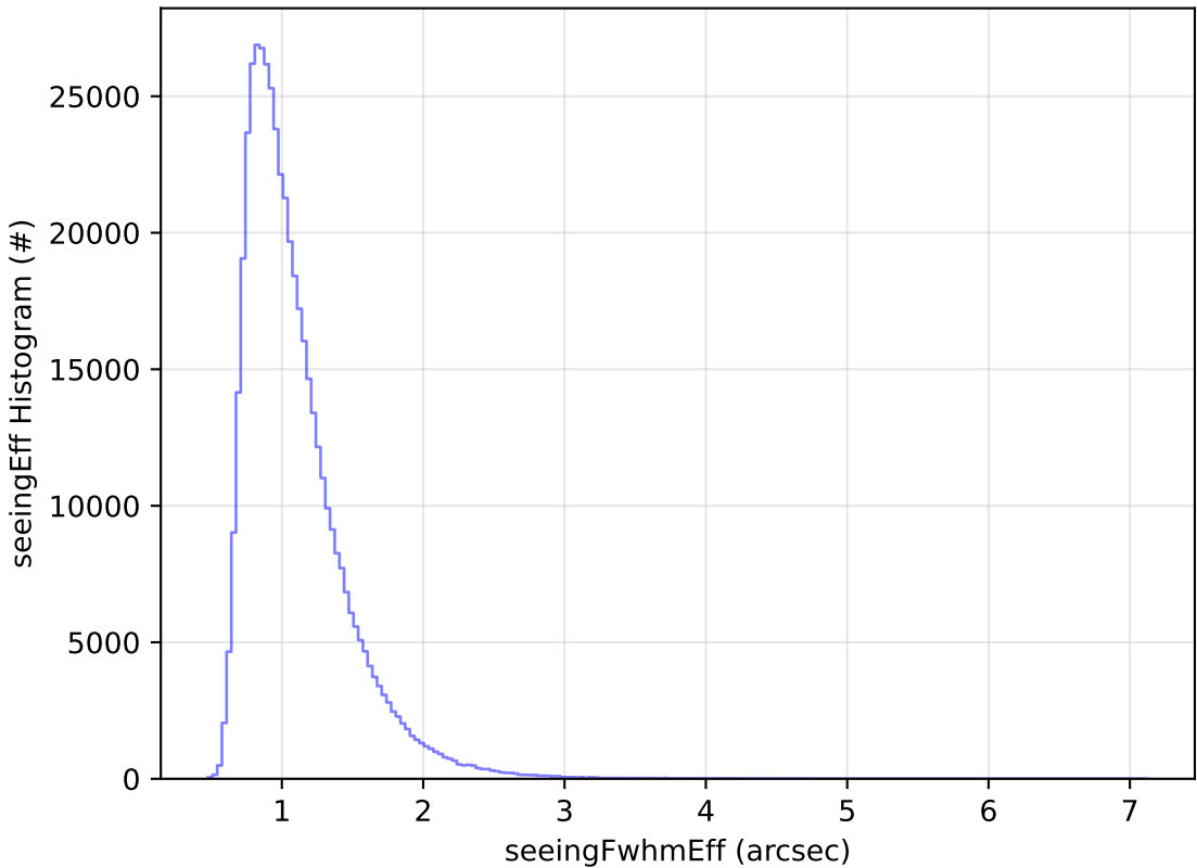
too_elab_r128_d3_gz_v3.4_10yrs WFD i band: seeingEff Histogram
