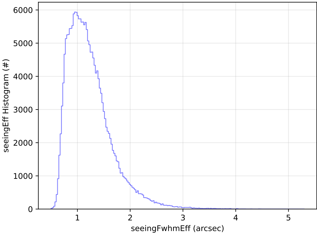
too_elab_r128_d3_gz_v3.4_10yrs WFD g band: seeingEff Histogram
