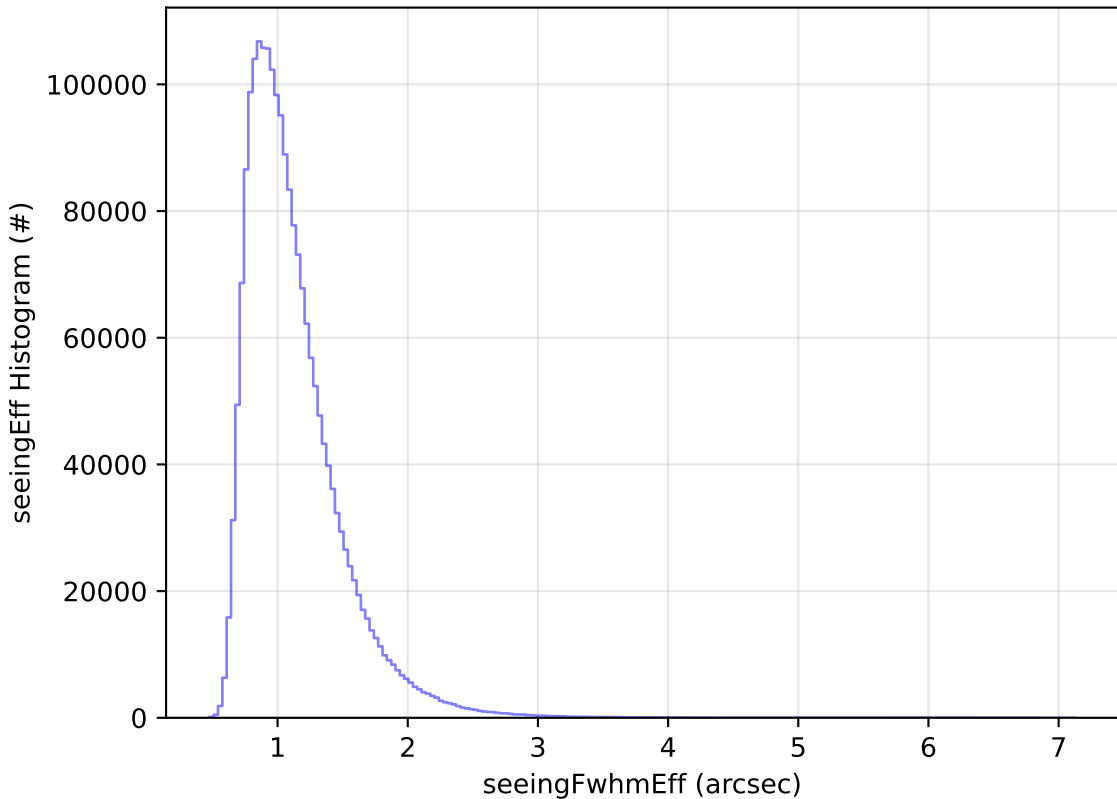
too_elab_r128_d3_gz_v3.4_10yrs WFD all bands: seeingEff Histogram
