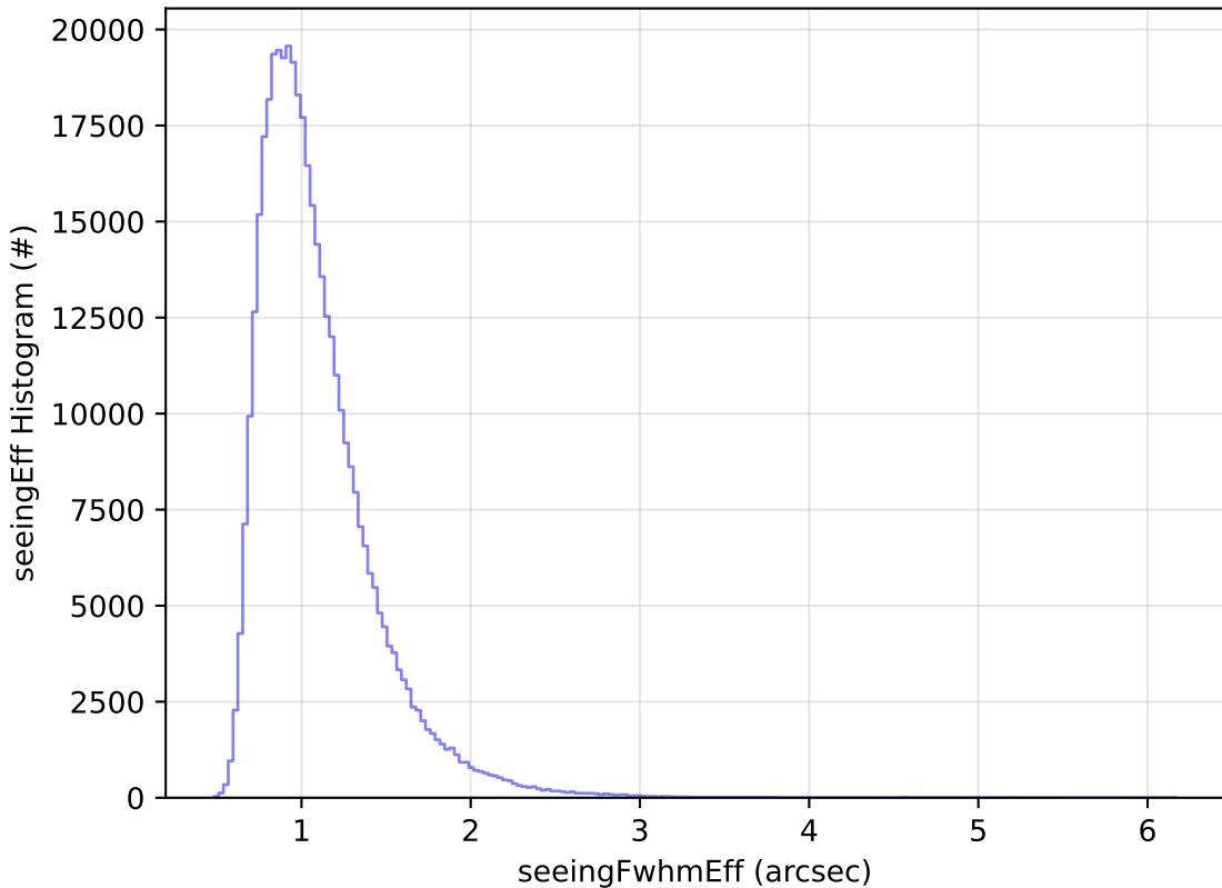
too_elab_r128_d3_gz_v3.4_10yrs All sky z band: seeingEff Histogram
