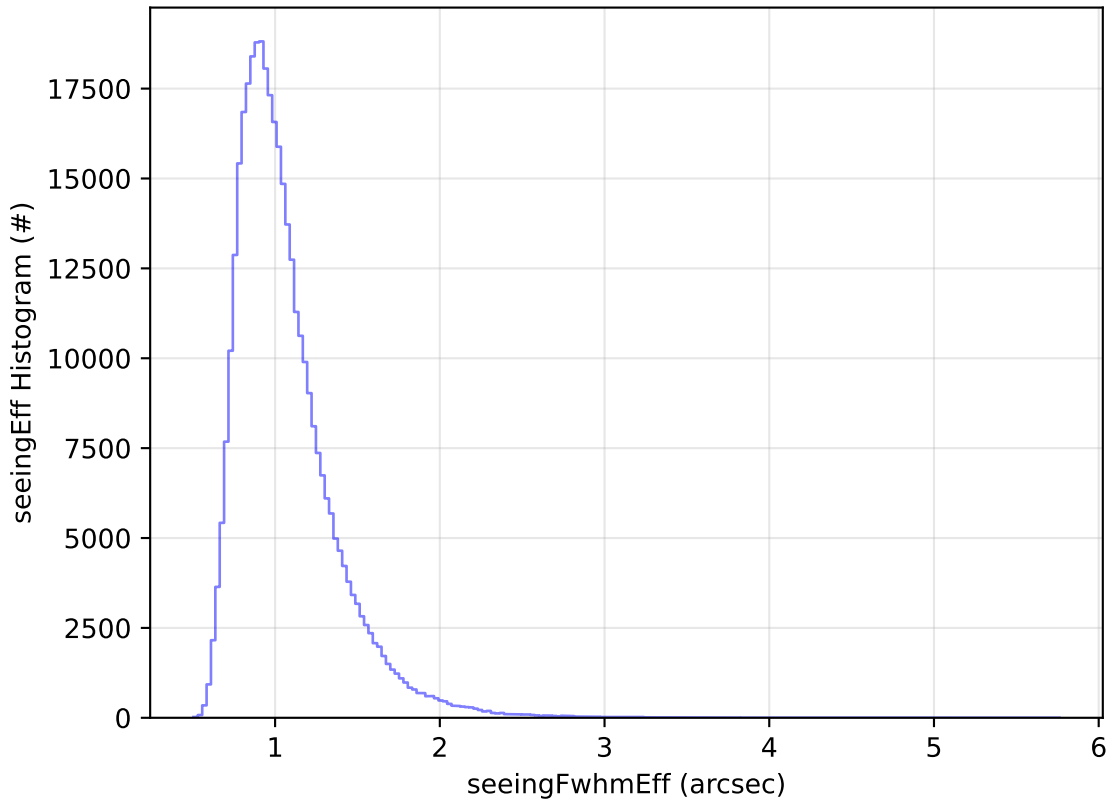
too_elab_r128_d3_gz_v3.4_10yrs All sky y band: seeingEff Histogram
