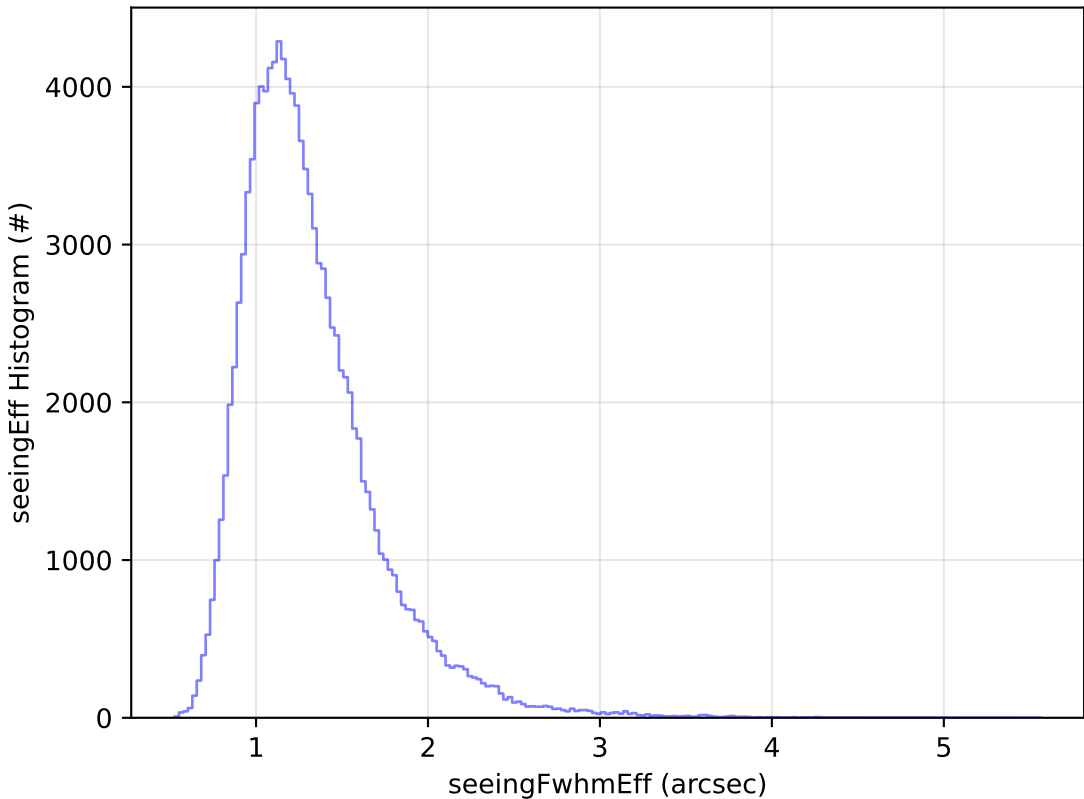
too_elab_r128_d3_gz_v3.4_10yrs All sky u band: seeingEff Histogram
