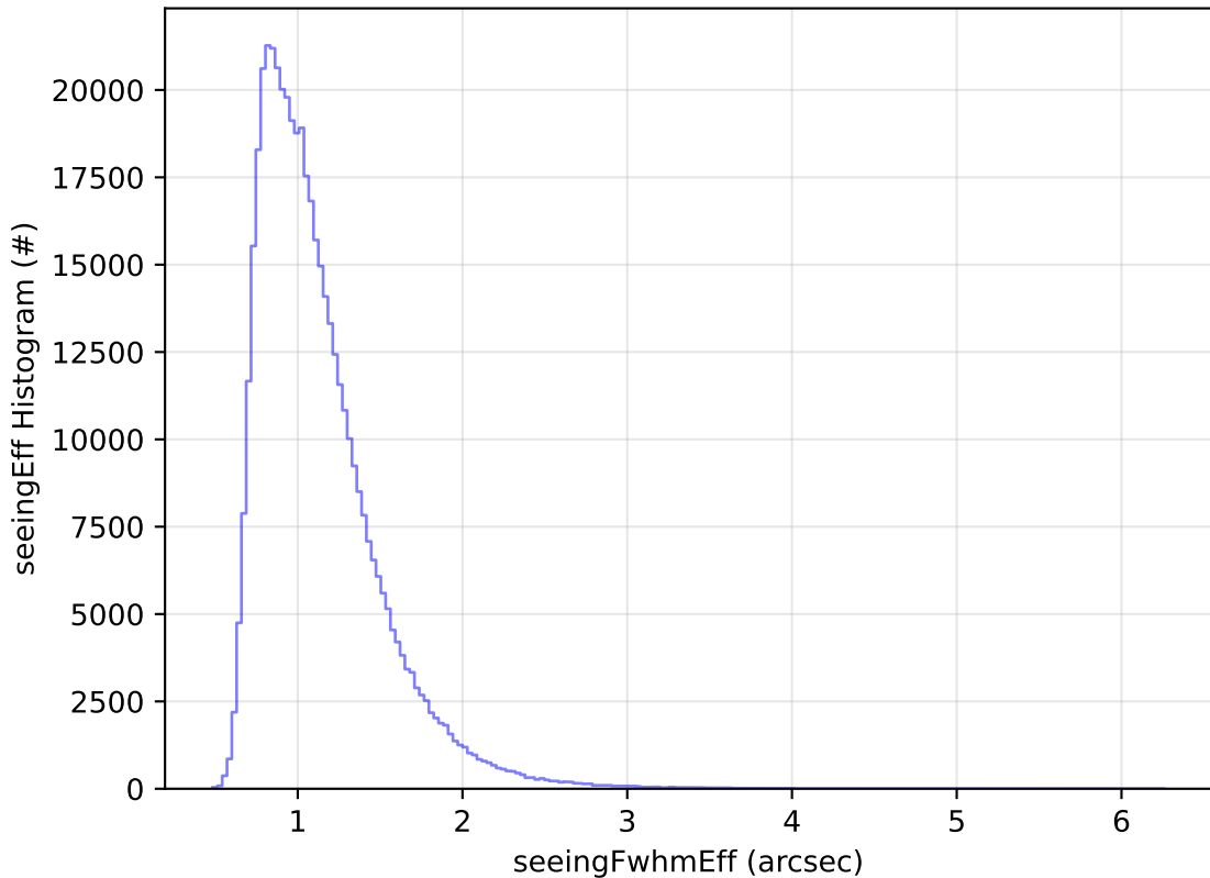
too_elab_r128_d3_gz_v3.4_10yrs All sky r band: seeingEff Histogram
