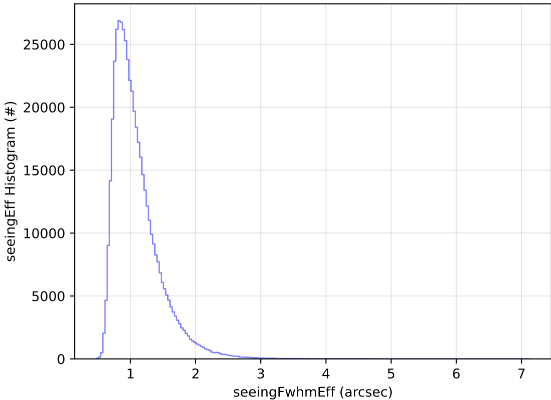
too_elab_r128_d3_gz_v3.4_10yrs All sky i band: seeingEff Histogram
