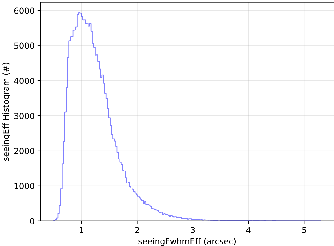
too_elab_r128_d3_gz_v3.4_10yrs All sky g band: seeingEff Histogram
