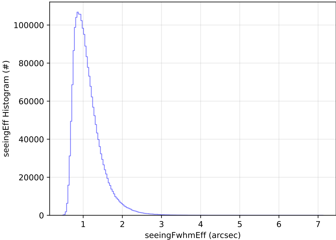
too_elab_r128_d3_gz_v3.4_10yrs All sky all bands: seeingEff Histogram
