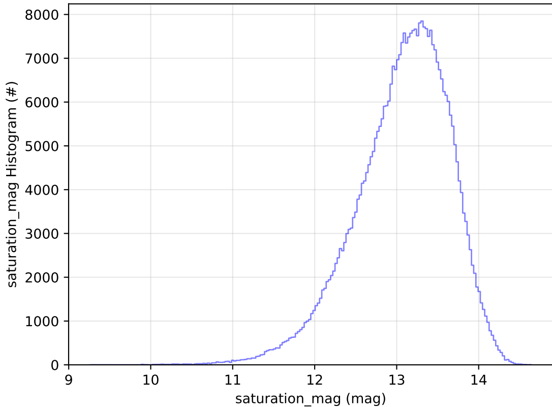
too_elab_r128_d3_gz_v3.4_10yrs WFD y band: saturation_mag Histogram
