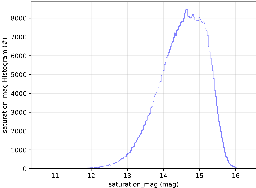
too_elab_r128_d3_gz_v3.4_10yrs WFD r band: saturation_mag Histogram
