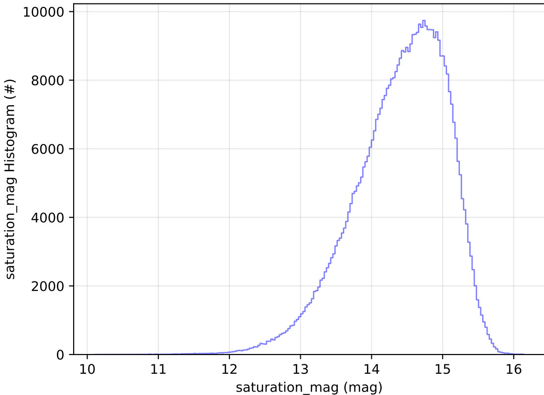
too_elab_r128_d3_gz_v3.4_10yrs WFD i band: saturation_mag Histogram
