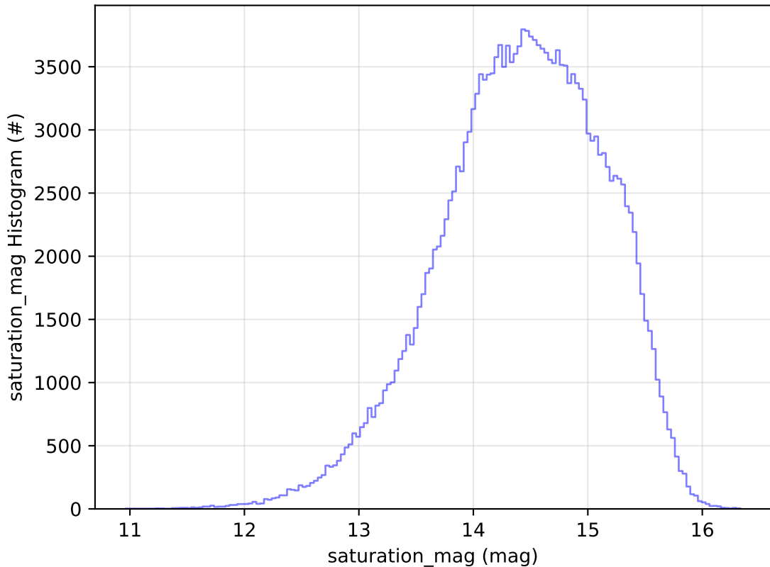
too_elab_r128_d3_gz_v3.4_10yrs WFD g band: saturation_mag Histogram
