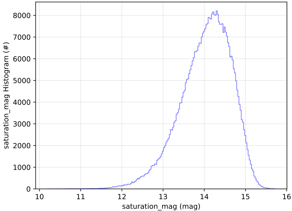
too_elab_r128_d3_gz_v3.4_10yrs All sky z band: saturation_mag Histogram
