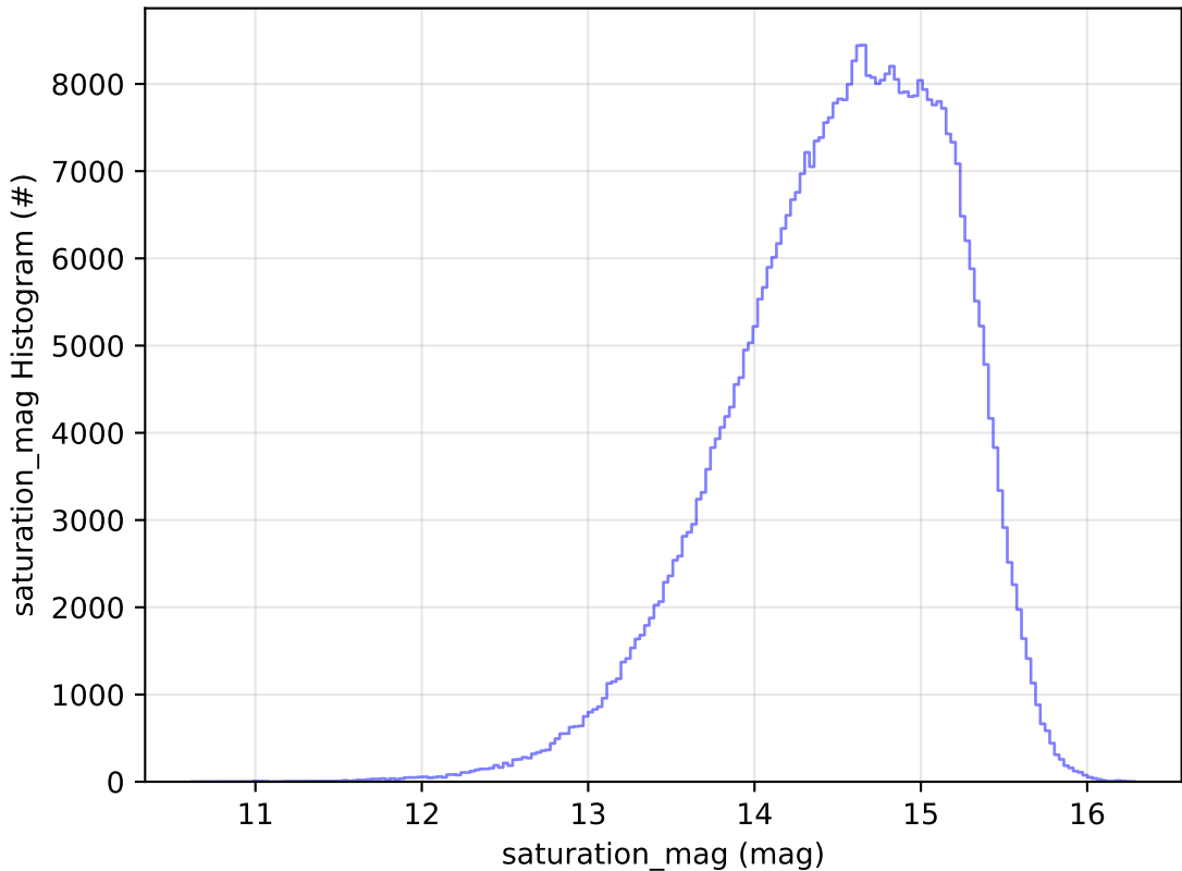
too_elab_r128_d3_gz_v3.4_10yrs All sky r band: saturation_mag Histogram
