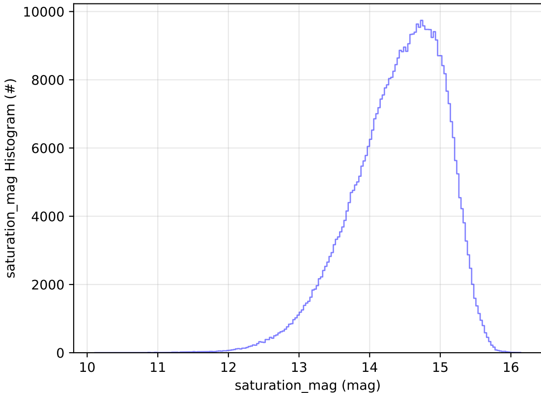
too_elab_r128_d3_gz_v3.4_10yrs All sky i band: saturation_mag Histogram
