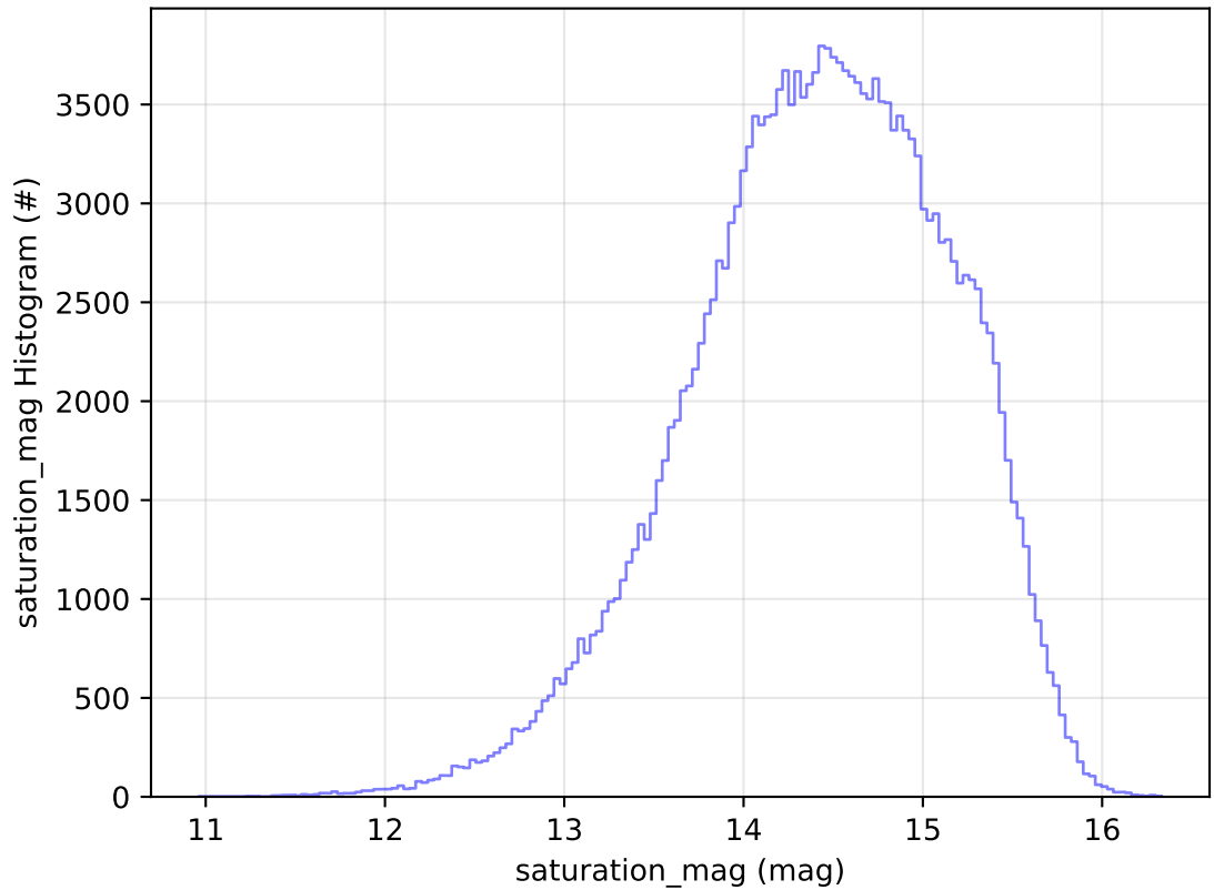
too_elab_r128_d3_gz_v3.4_10yrs All sky g band: saturation_mag Histogram
