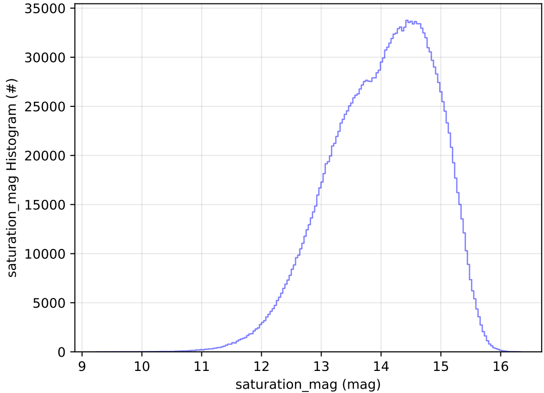
too_elab_r128_d3_gz_v3.4_10yrs All sky all bands: saturation_mag Histogram
