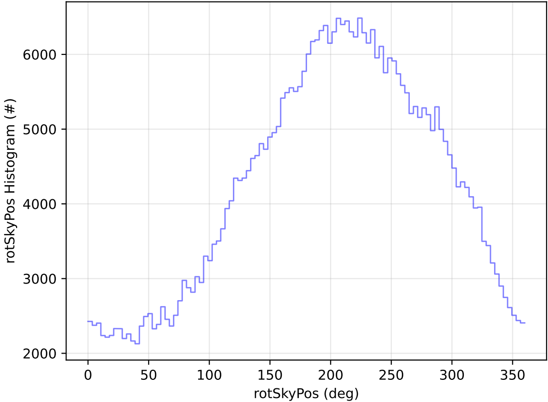
too_elab_r128_d3_gz_v3.4_10yrs WFD z band: rotSkyPos Histogram
