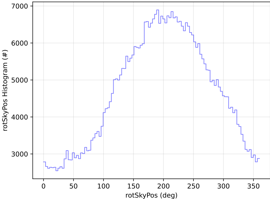
too_elab_r128_d3_gz_v3.4_10yrs WFD r band: rotSkyPos Histogram
