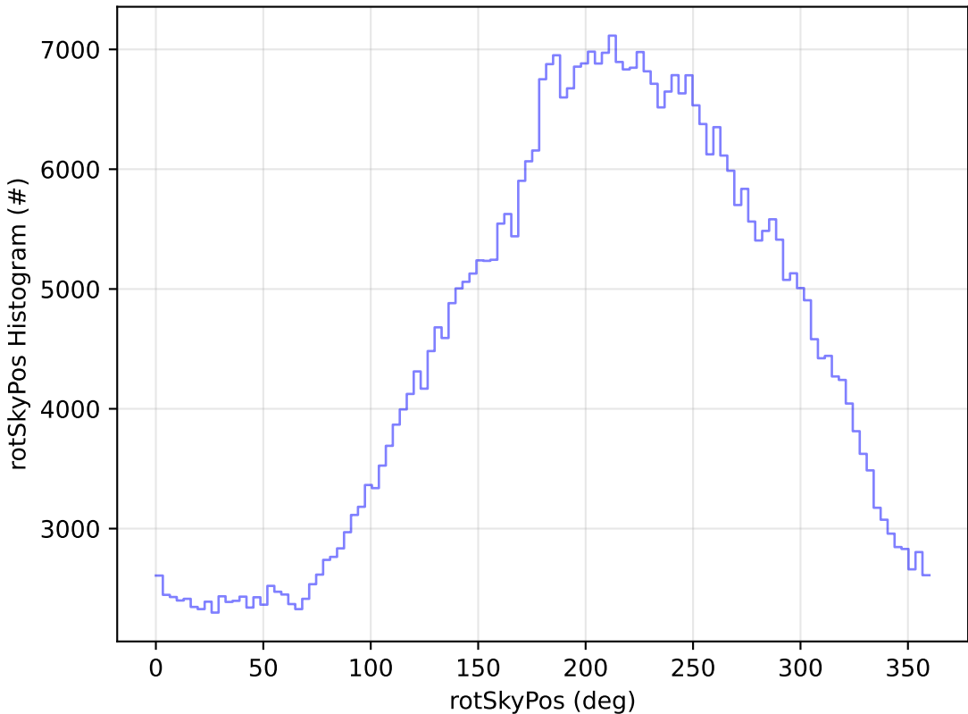
too_elab_r128_d3_gz_v3.4_10yrs WFD i band: rotSkyPos Histogram
