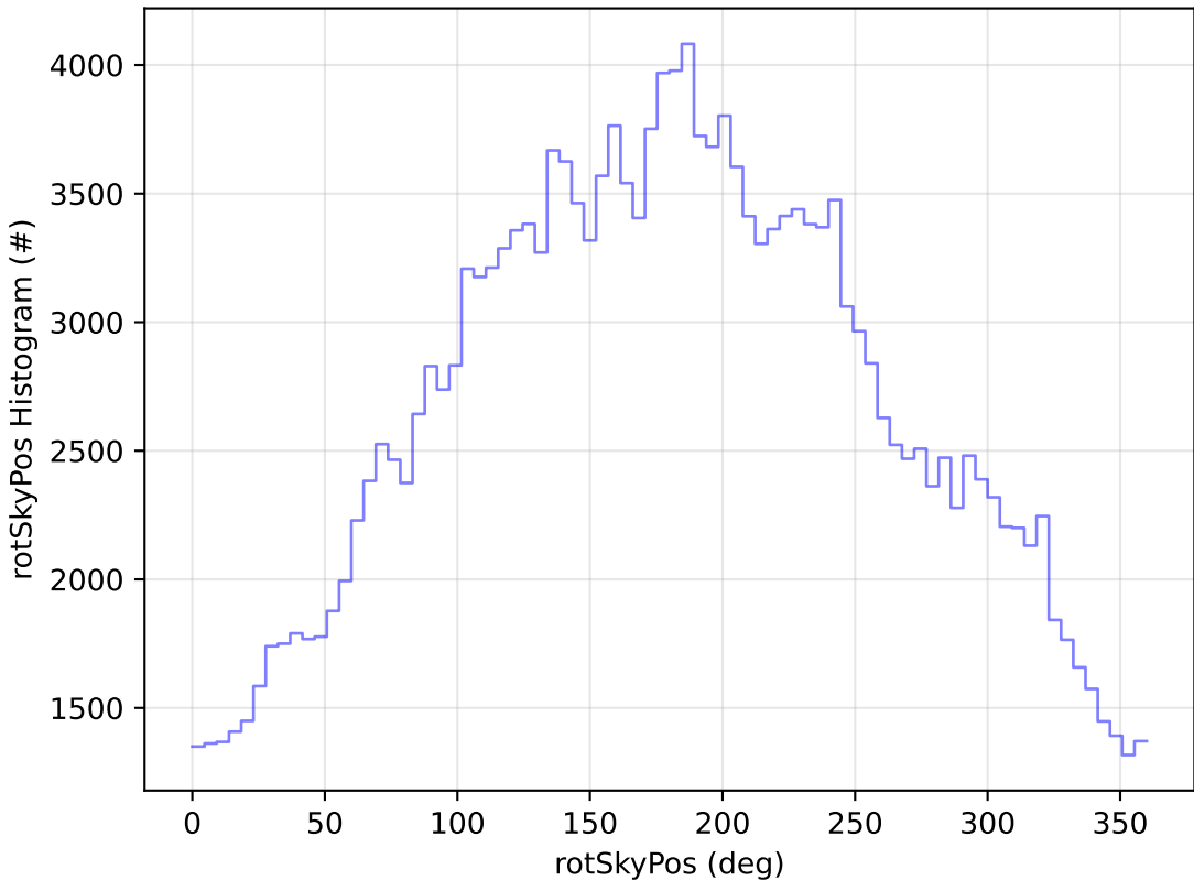
too_elab_r128_d3_gz_v3.4_10yrs WFD g band: rotSkyPos Histogram
