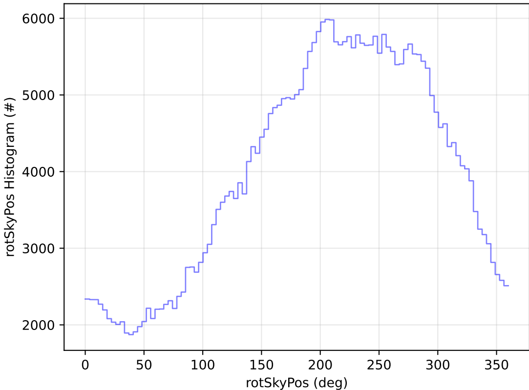
too_elab_r128_d3_gz_v3.4_10yrs All sky y band: rotSkyPos Histogram
