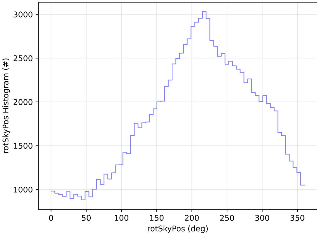
too_elab_r128_d3_gz_v3.4_10yrs All sky u band: rotSkyPos Histogram
